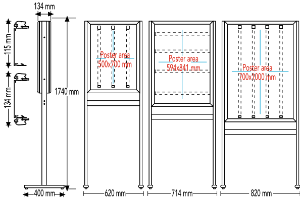
EXTRUSION: SILVER COLOR (ANODIZED) ALUMINIUM - FRAME PROFILE: 32 mm
